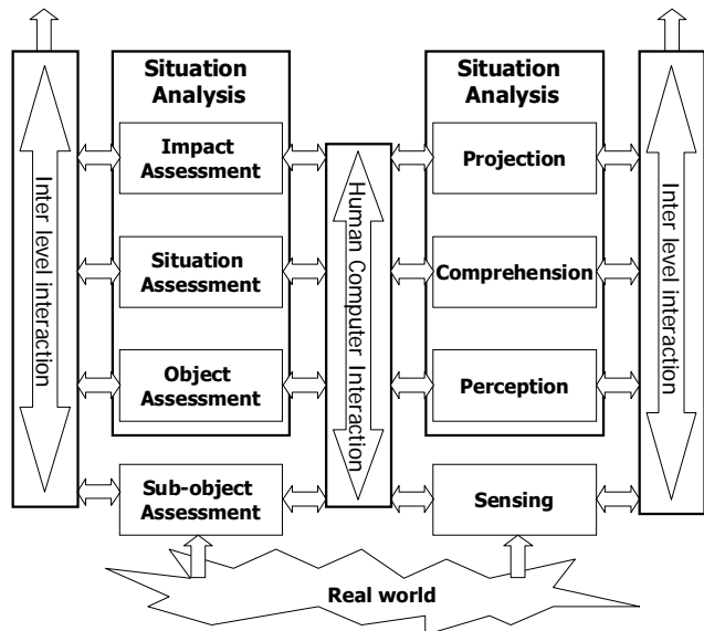
Figure 7: The unified model for Situation Analysis.
