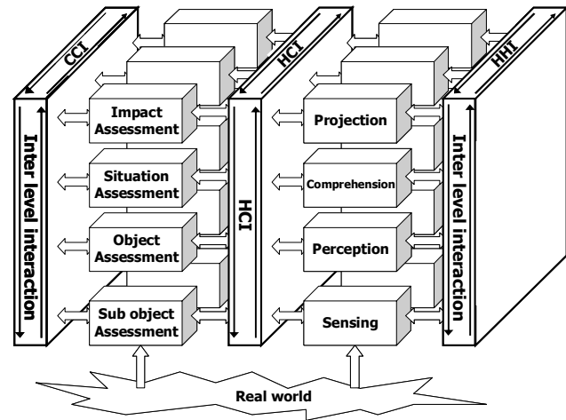
Figure 8: SA involving multiple machines interacting with multiple humans.
