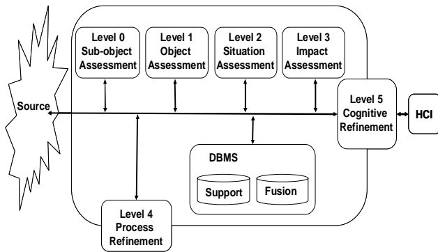
Figure 2: The JDL model (adapted from [11]).
