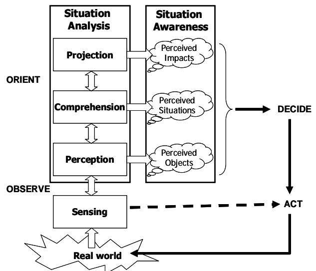
Figure 5 : The OODA loop added to Figure 4 (human perspective). Observe and orient are parts of the SA process. The result of this process, i.e., SAW, is used as basis for decision making.
